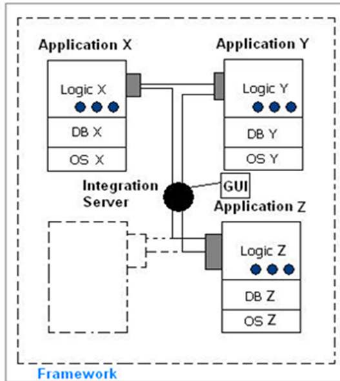
Fig. 2. Process integration
