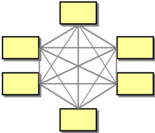
Fig. 4. Point-to-point integration
