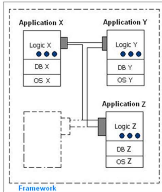
Fig. 1. Application integration
