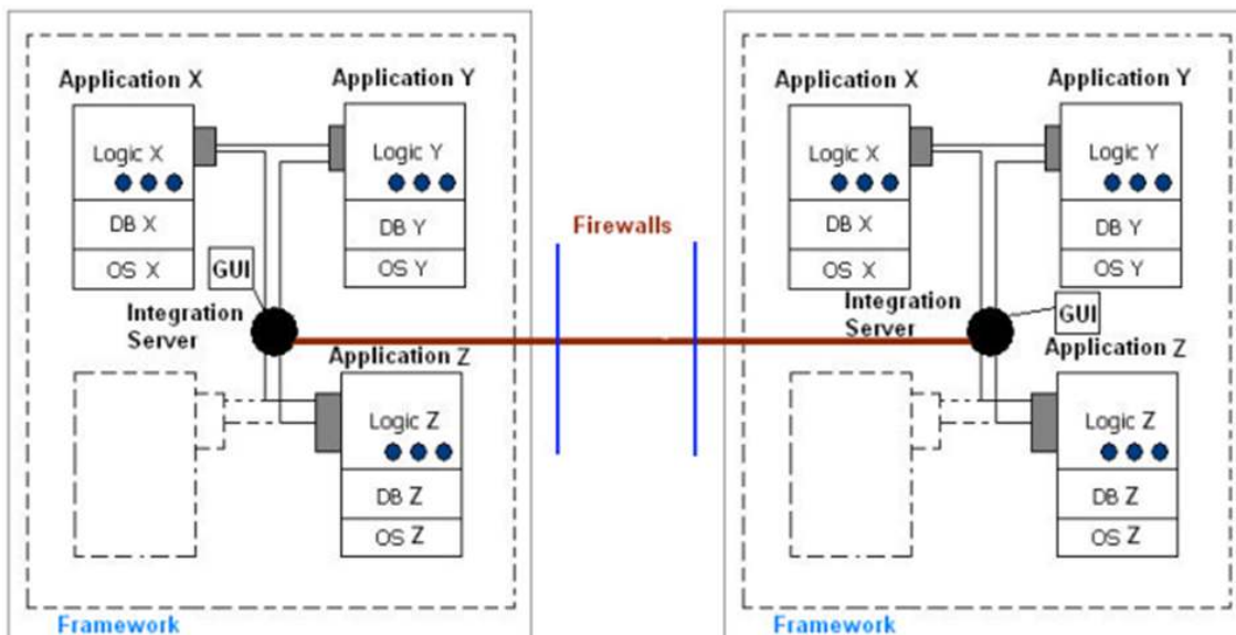
Fig. 3. B2B integration
